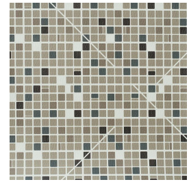
Pattern: Streets
